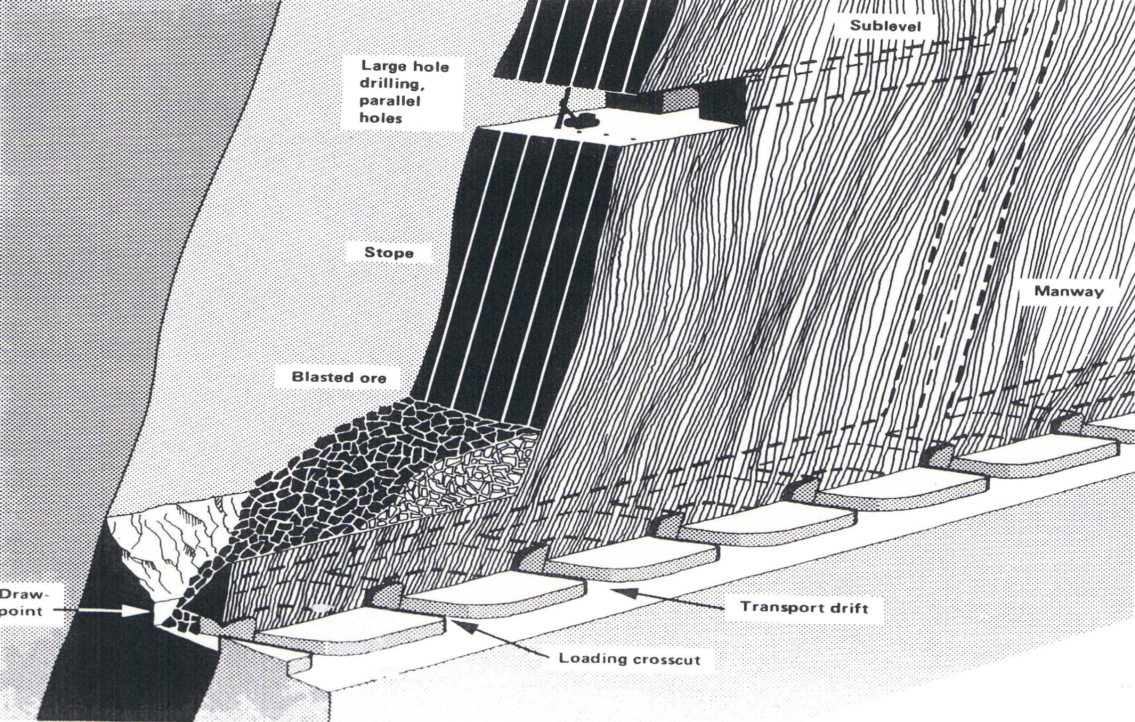
Sublevel stoping with large-hole drilling and blasting.
