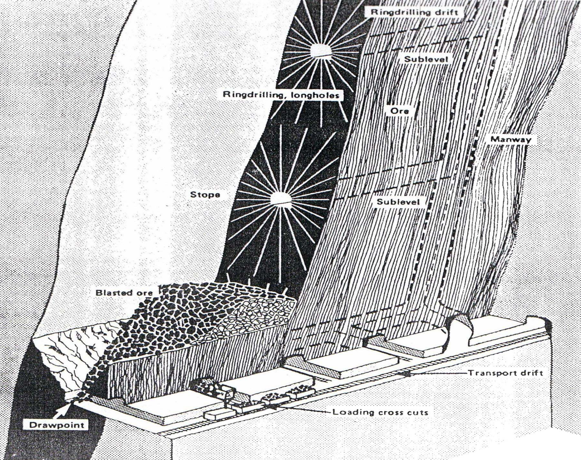
Sublevel stoping with ring drilling as the primary means of breaking ore.
