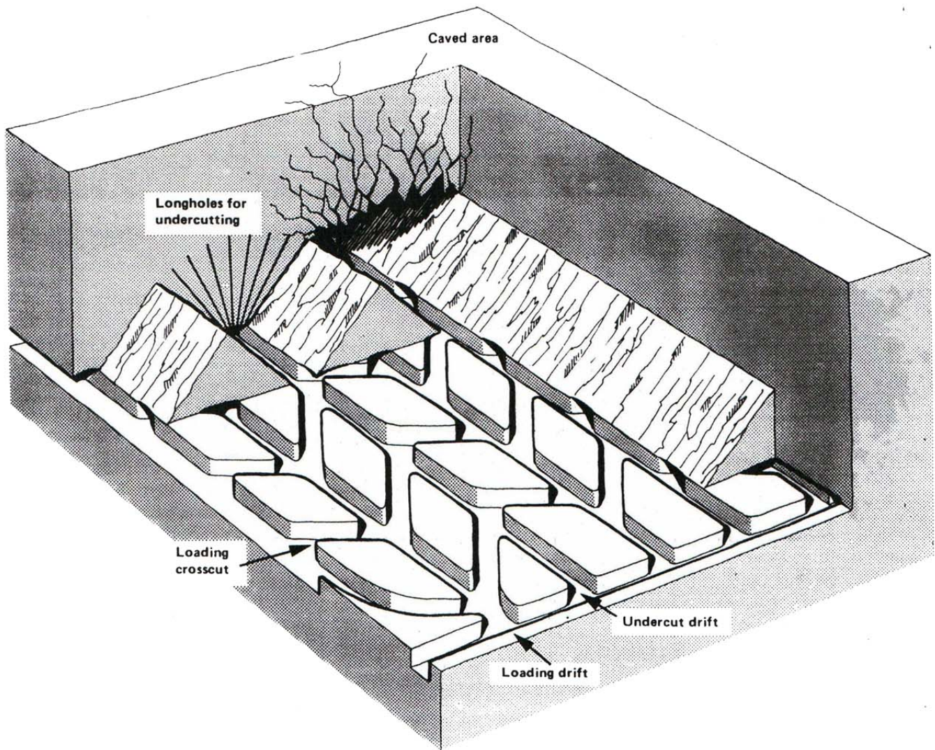
Block caving in a massive ore body, showing the layout for trackless mining.
