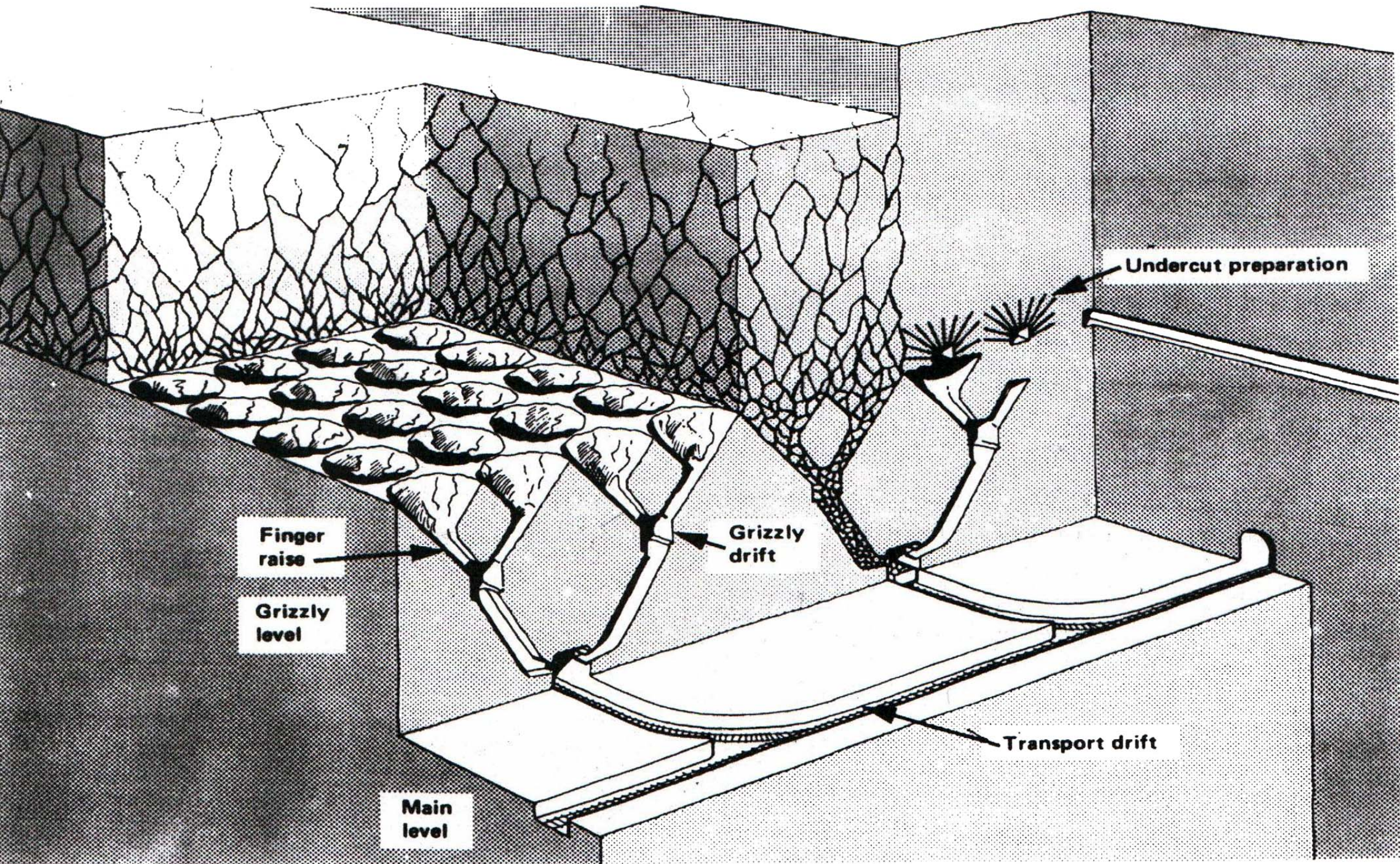
Block caving in a massive ore body, showing the conventional mining layout.
