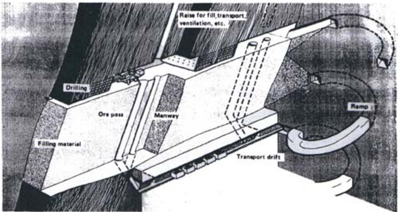
Cut-and-fill mining in a large vertical ore body.
