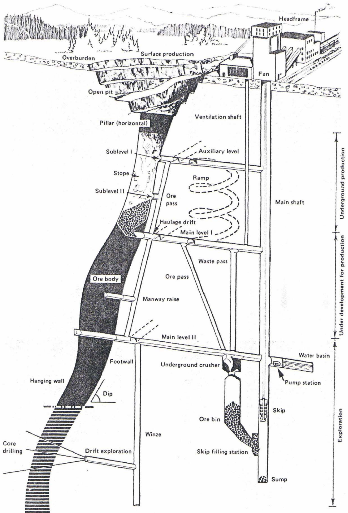
Sample layout of an underground mine, identifying various mining operations and terms.
