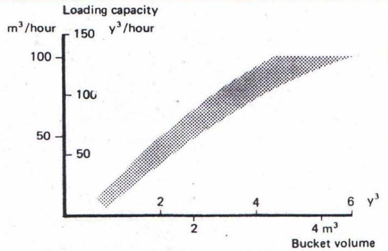
FRONT LOADER AND TRANSPORT VEHICLES
