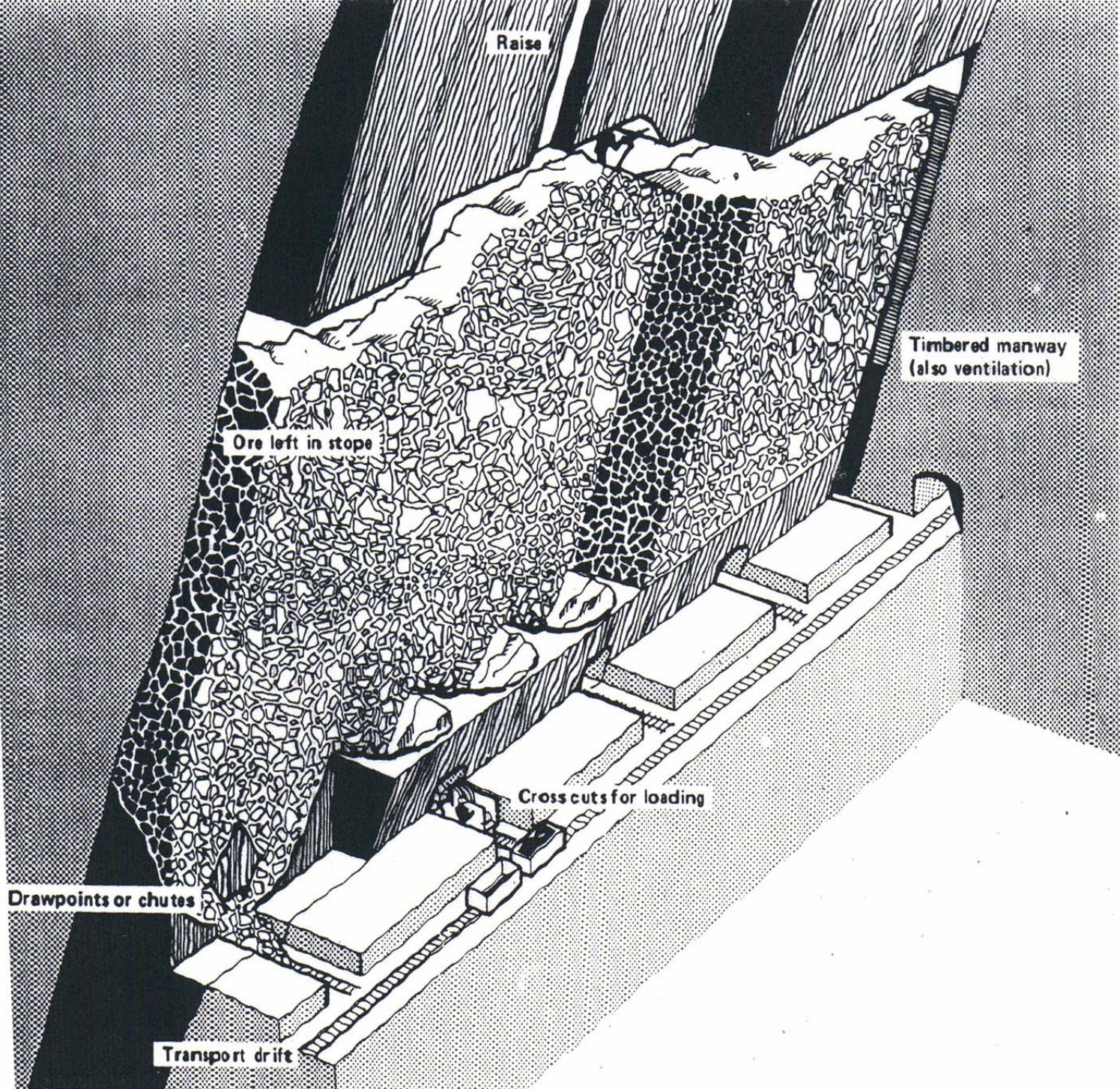
Shrinkage stoping in a large vertical ore body.
