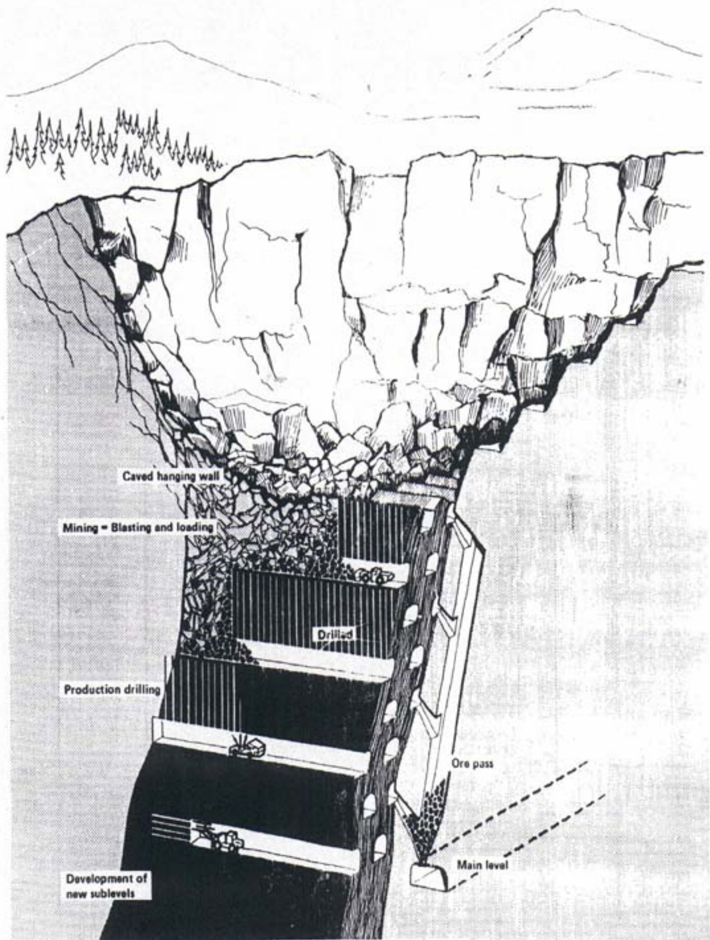
Sublevel caving in a large and steeply dipping ore body.
